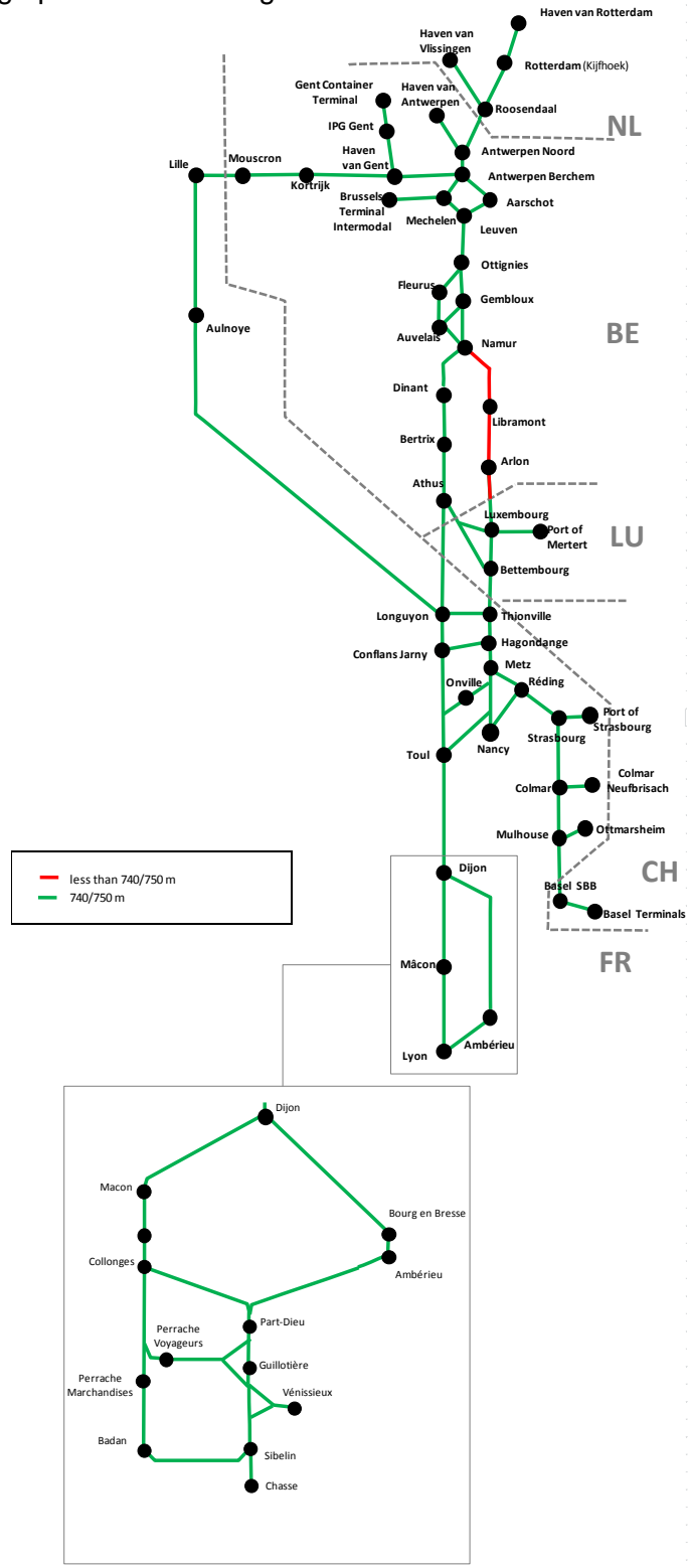
Map 8: maximum train length allowed
