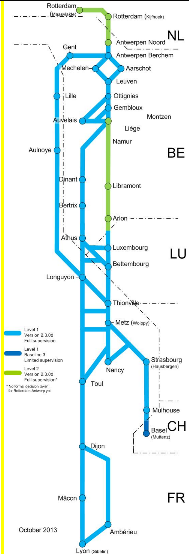
Map 22: nature of the ETCS deployment system along the corridor lines that were established in Nov. 2013
